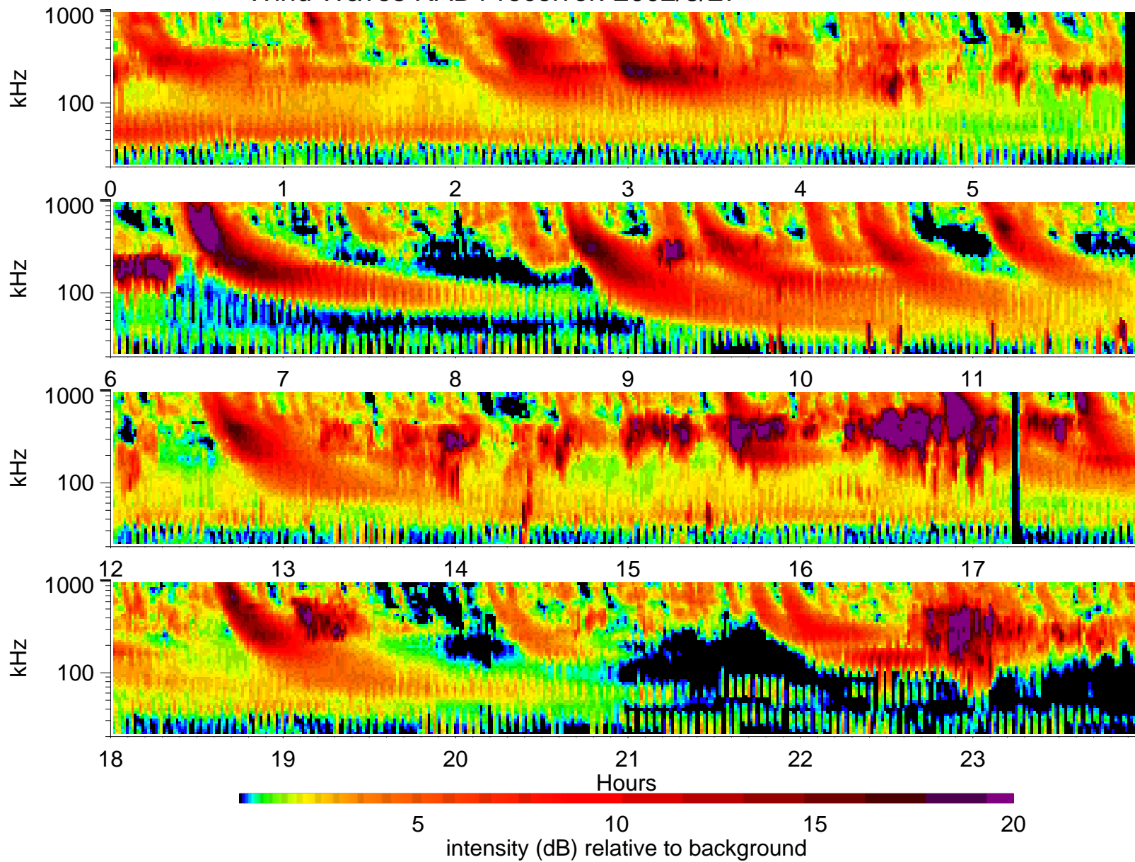
Wind Waves RAD1 receiver: 2002/8/27
