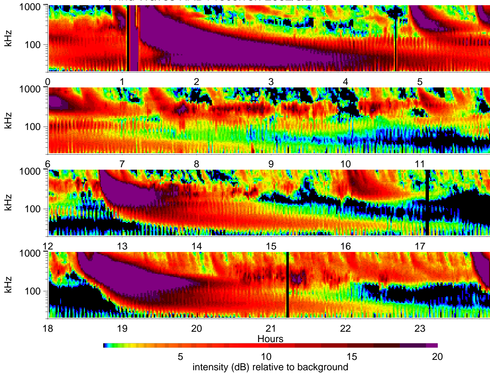
Wind Waves RAD1 receiver: 2002/8/24
