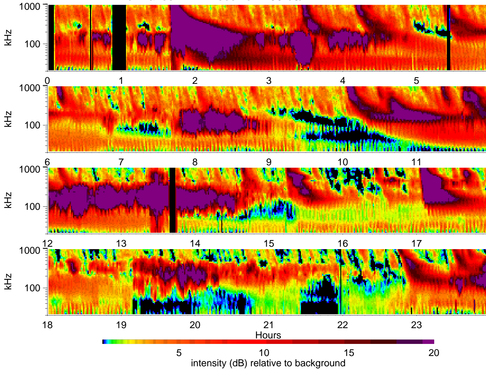
Wind Waves RAD1 receiver: 2002/8/21
