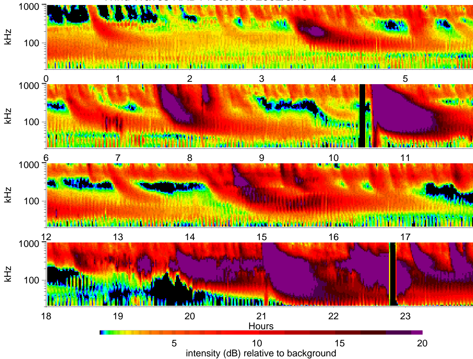
Wind Waves RAD1 receiver: 2002/8/19
