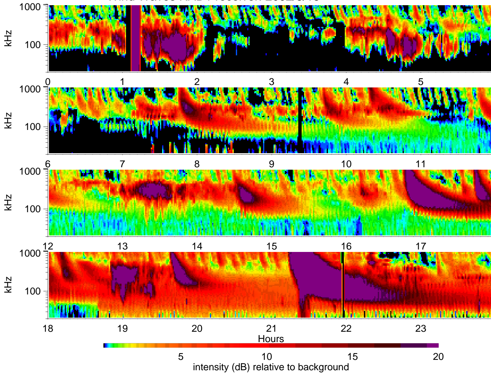
Wind Waves RAD1 receiver: 2002/8/18
