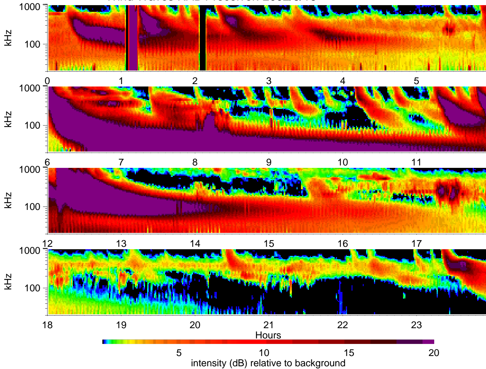
Wind Waves RAD1 receiver: 2002/8/16
