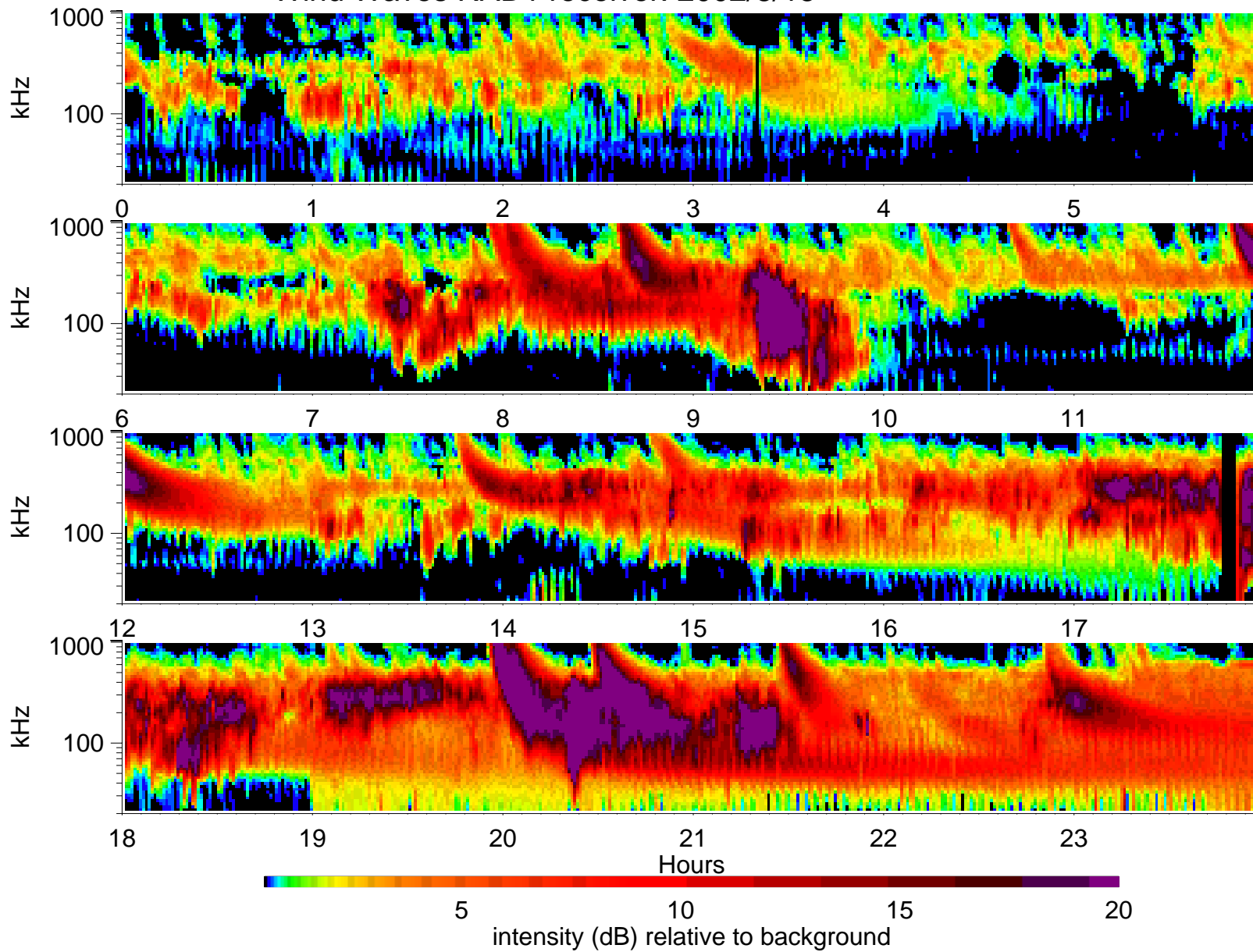
Wind Waves RAD1 receiver: 2002/8/15
