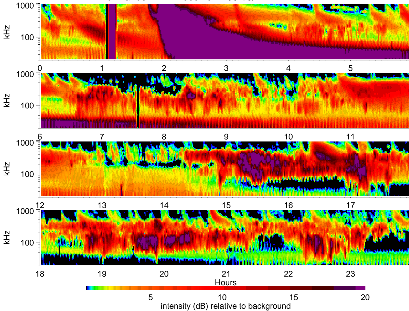
Wind Waves RAD1 receiver: 2002/8/14
