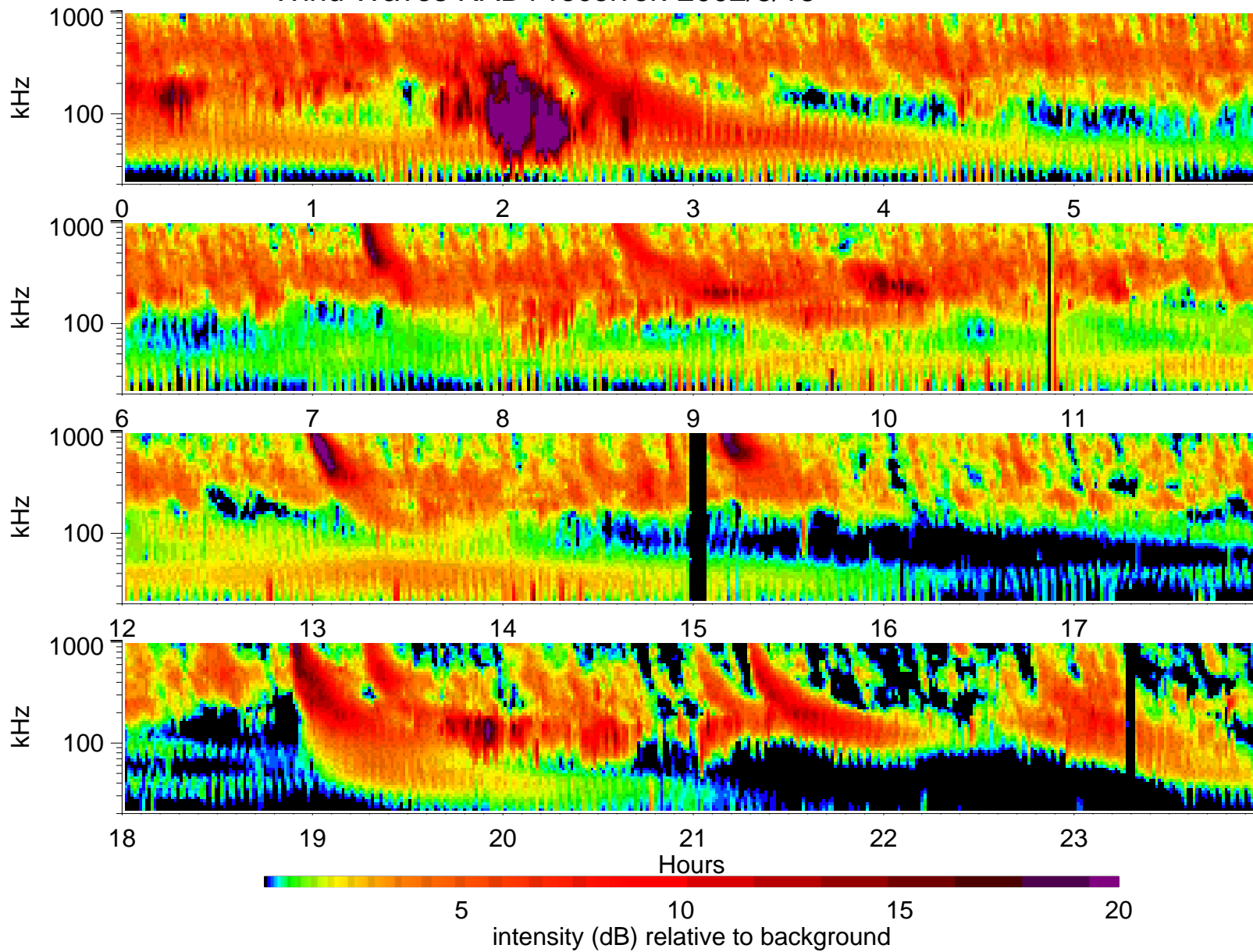
Wind Waves RAD1 receiver: 2002/8/13
