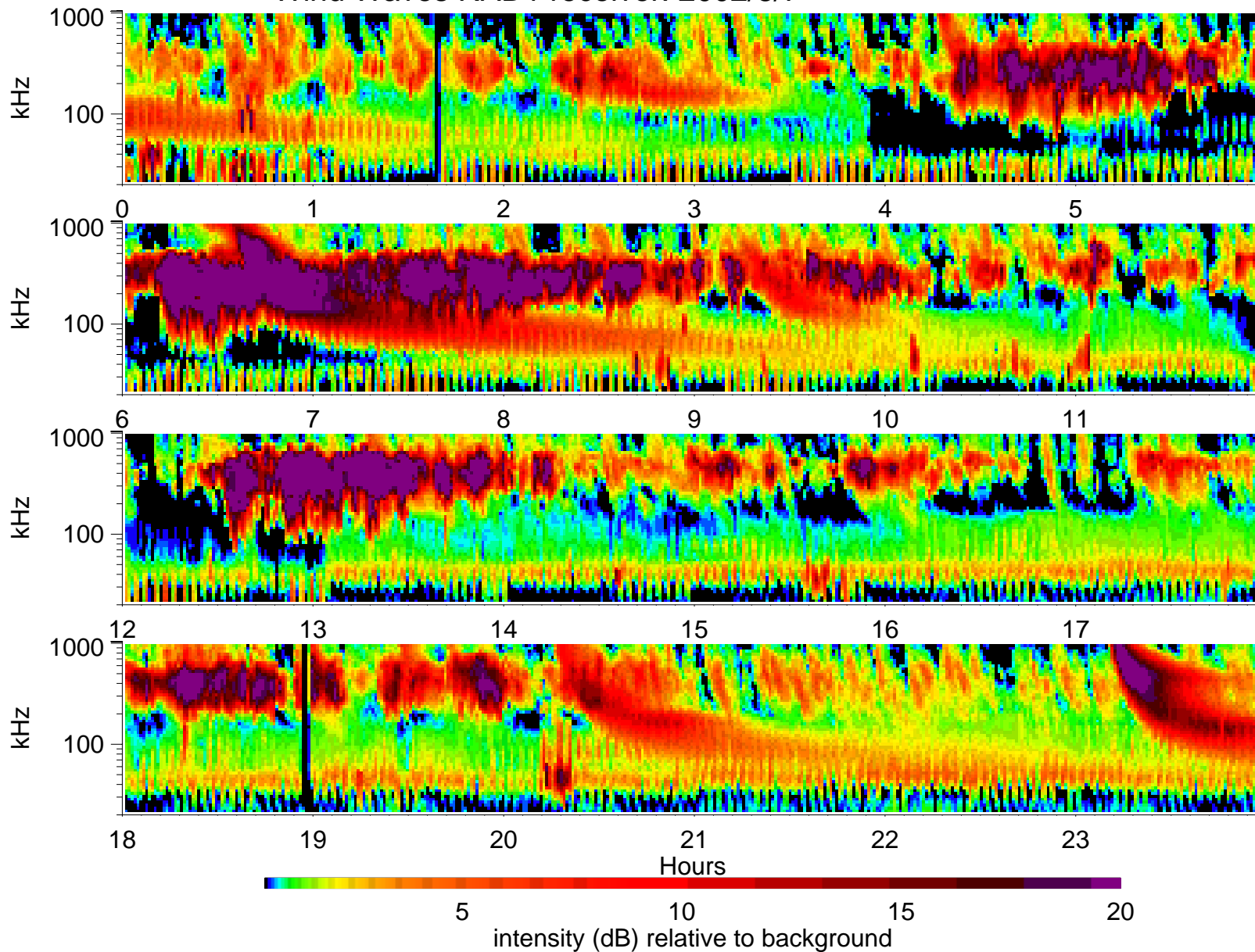
Wind Waves RAD1 receiver: 2002/8/7
