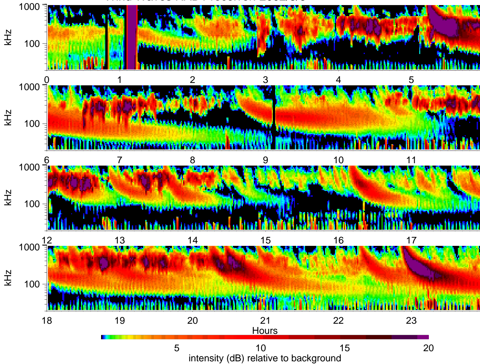
Wind Waves RAD1 receiver: 2002/8/6
