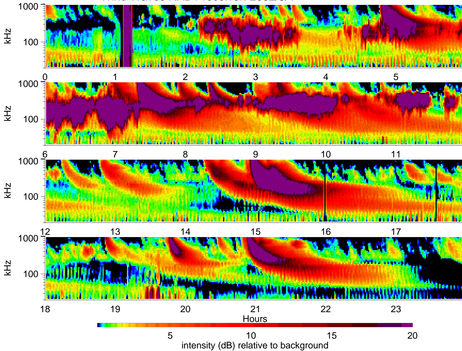
Wind Waves RAD1 receiver: 2002/8/4
