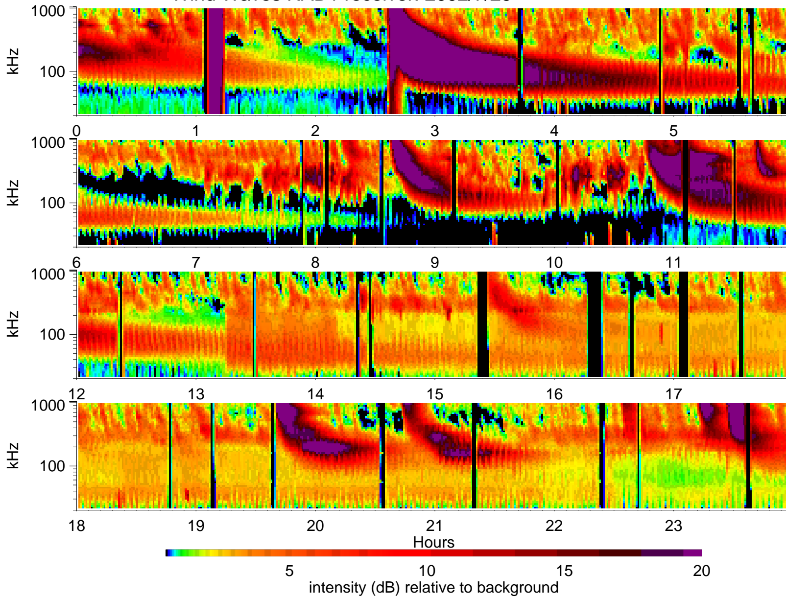
Wind Waves RAD1 receiver: 2002/7/29
