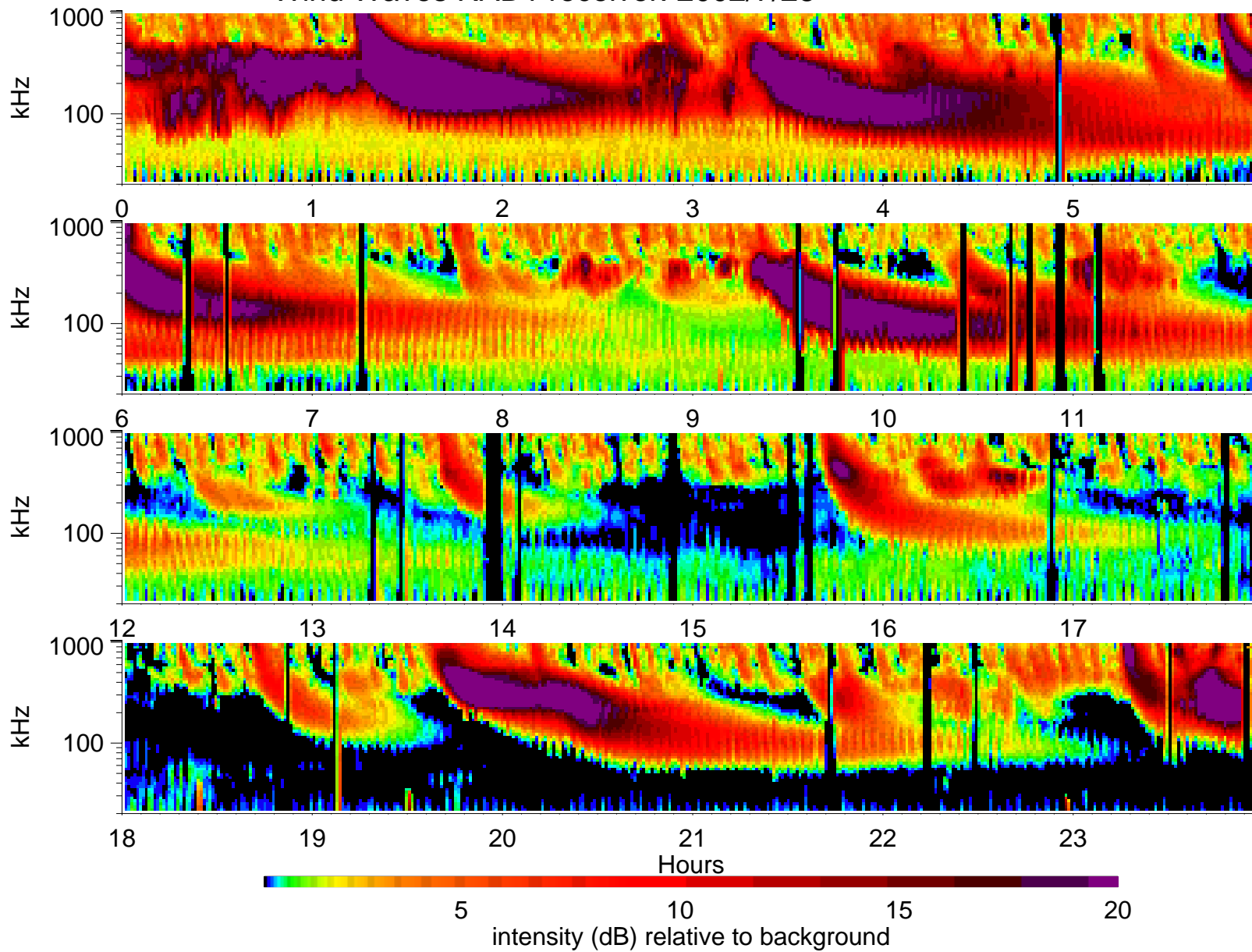
Wind Waves RAD1 receiver: 2002/7/28
