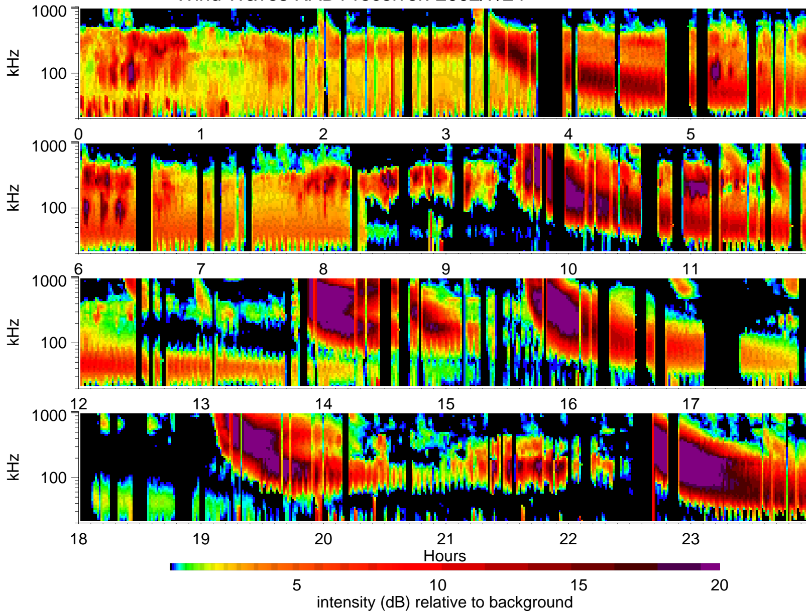
Wind Waves RAD1 receiver: 2002/7/24
