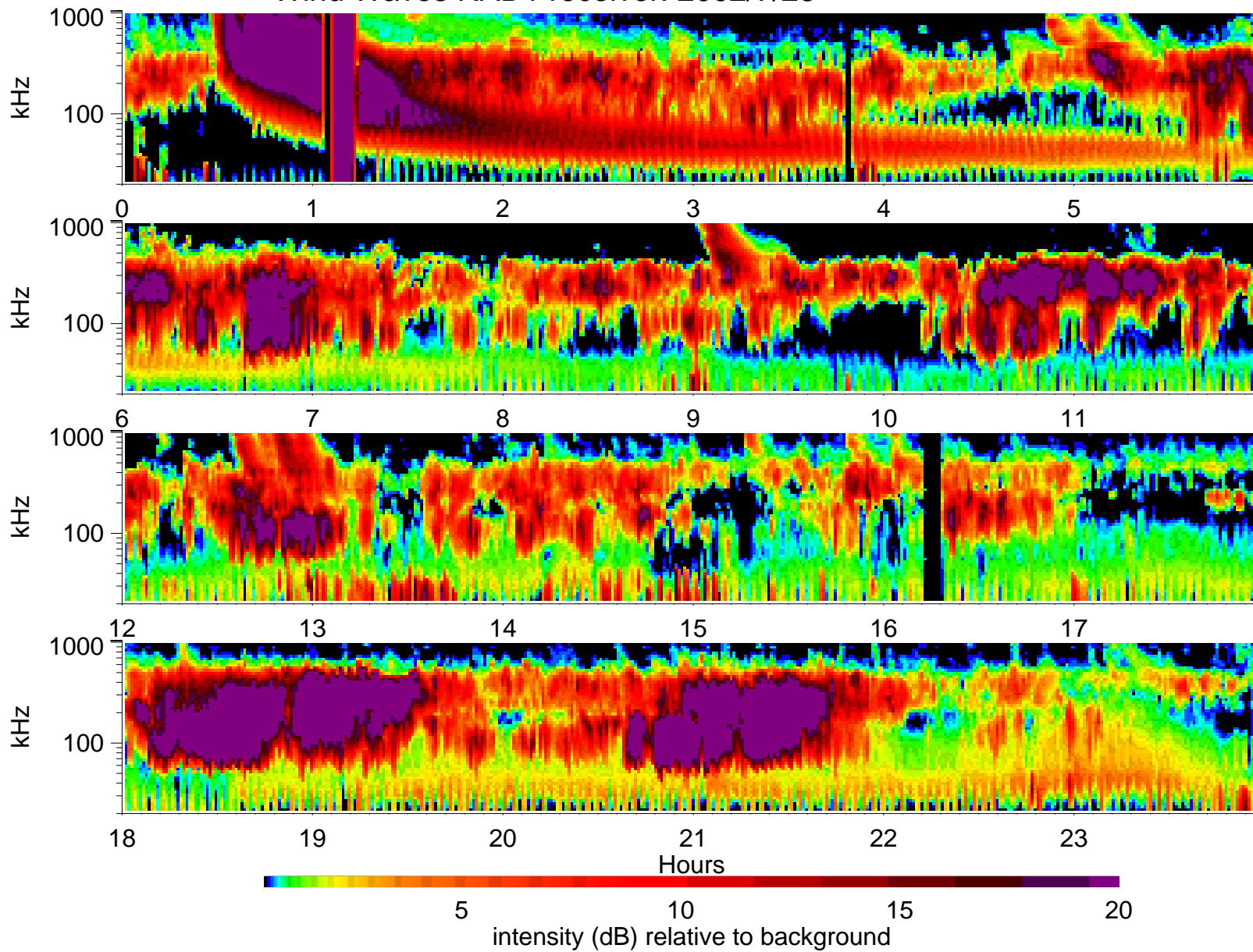
Wind Waves RAD1 receiver: 2002/7/23
