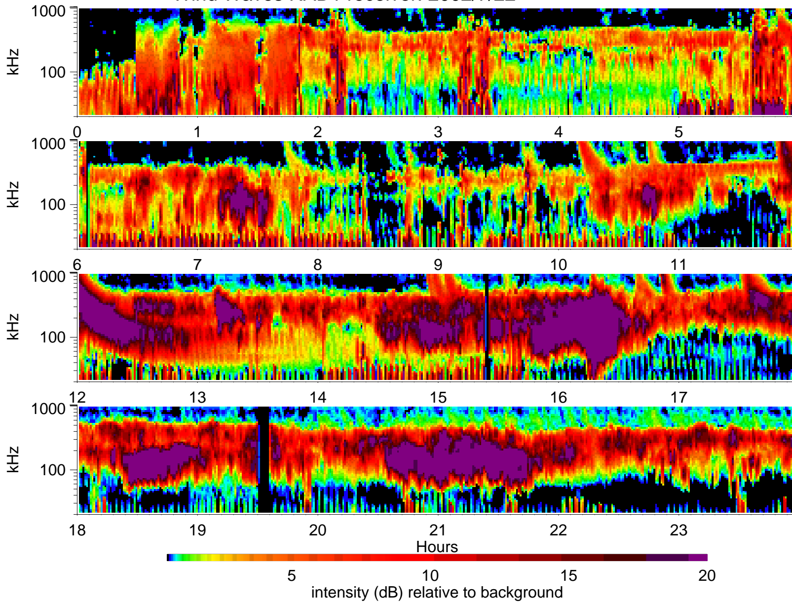
Wind Waves RAD1 receiver: 2002/7/22
