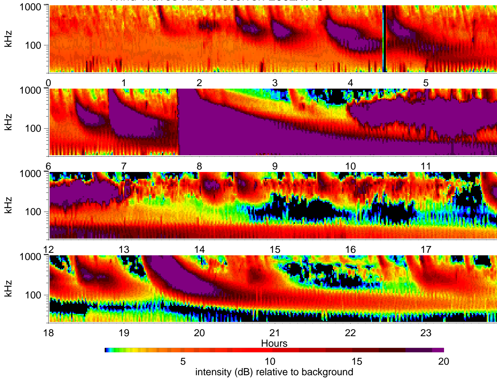
Wind Waves RAD1 receiver: 2002/7/18
