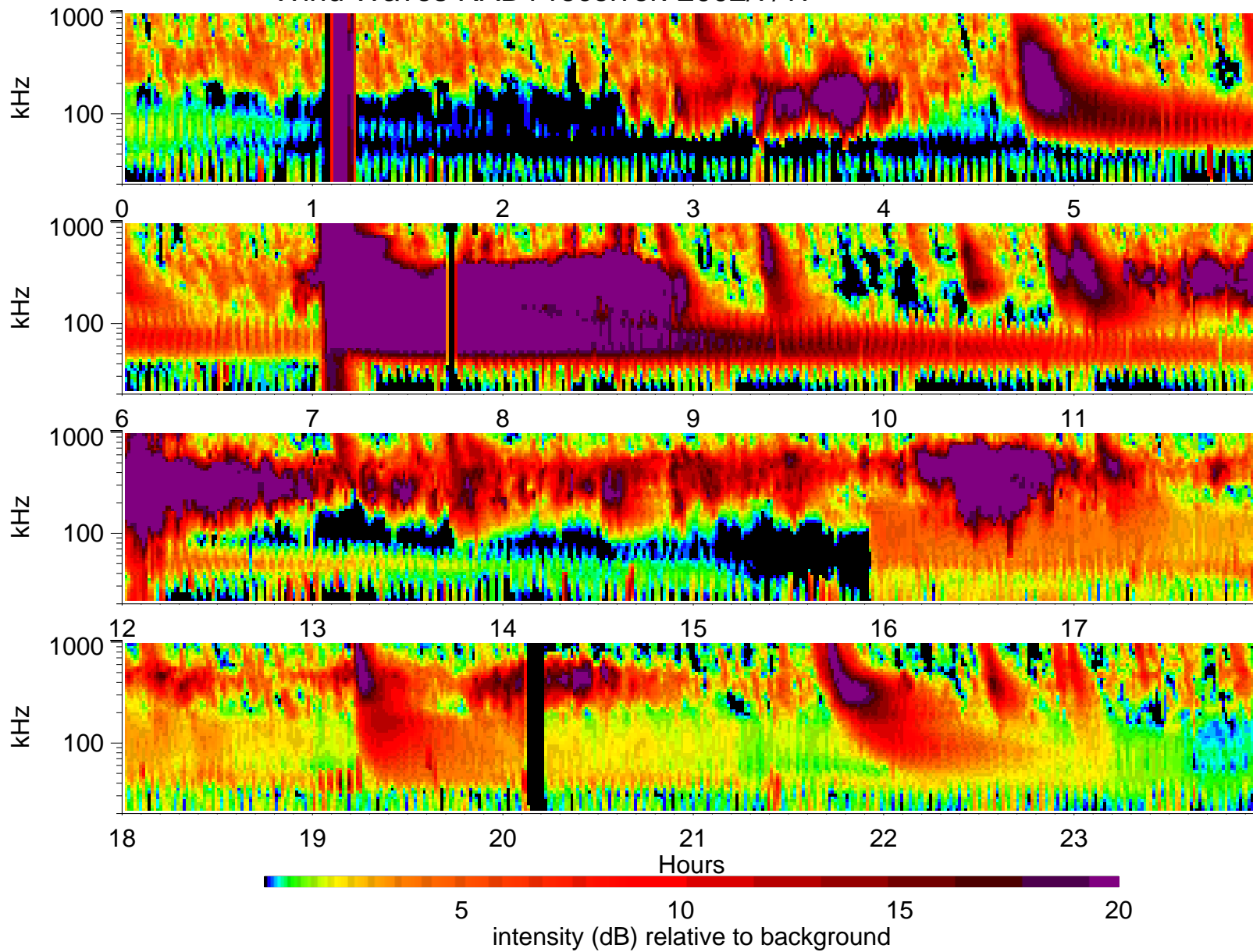
Wind Waves RAD1 receiver: 2002/7/17
