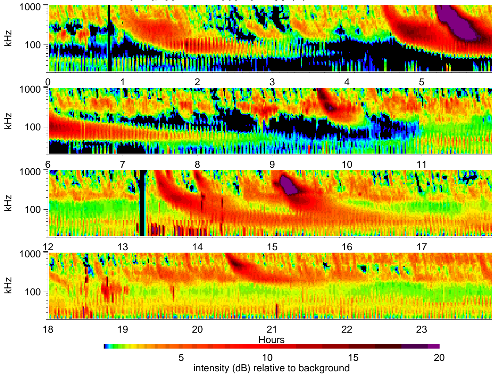
Wind Waves RAD1 receiver: 2002/7/14
