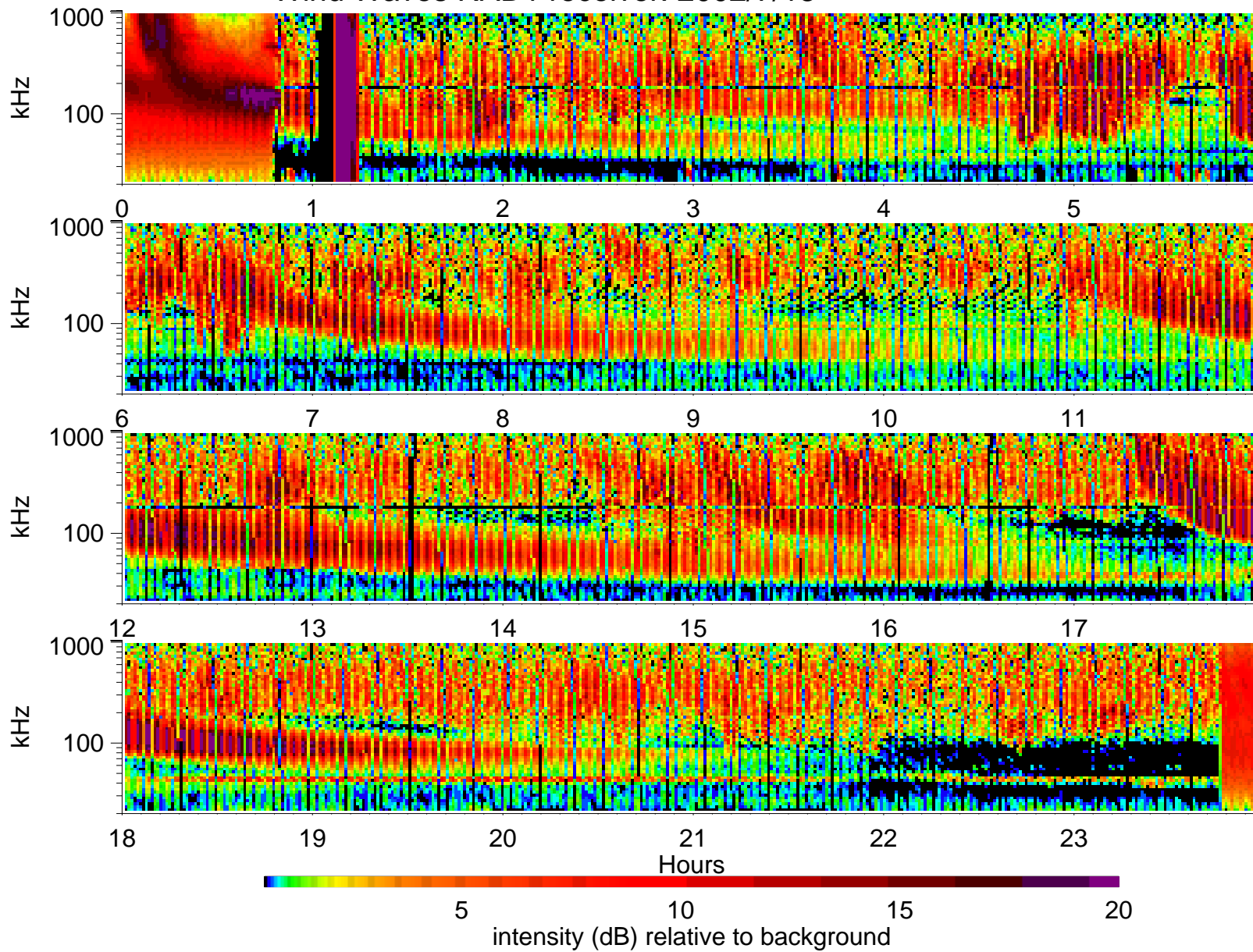
Wind Waves RAD1 receiver: 2002/7/13
