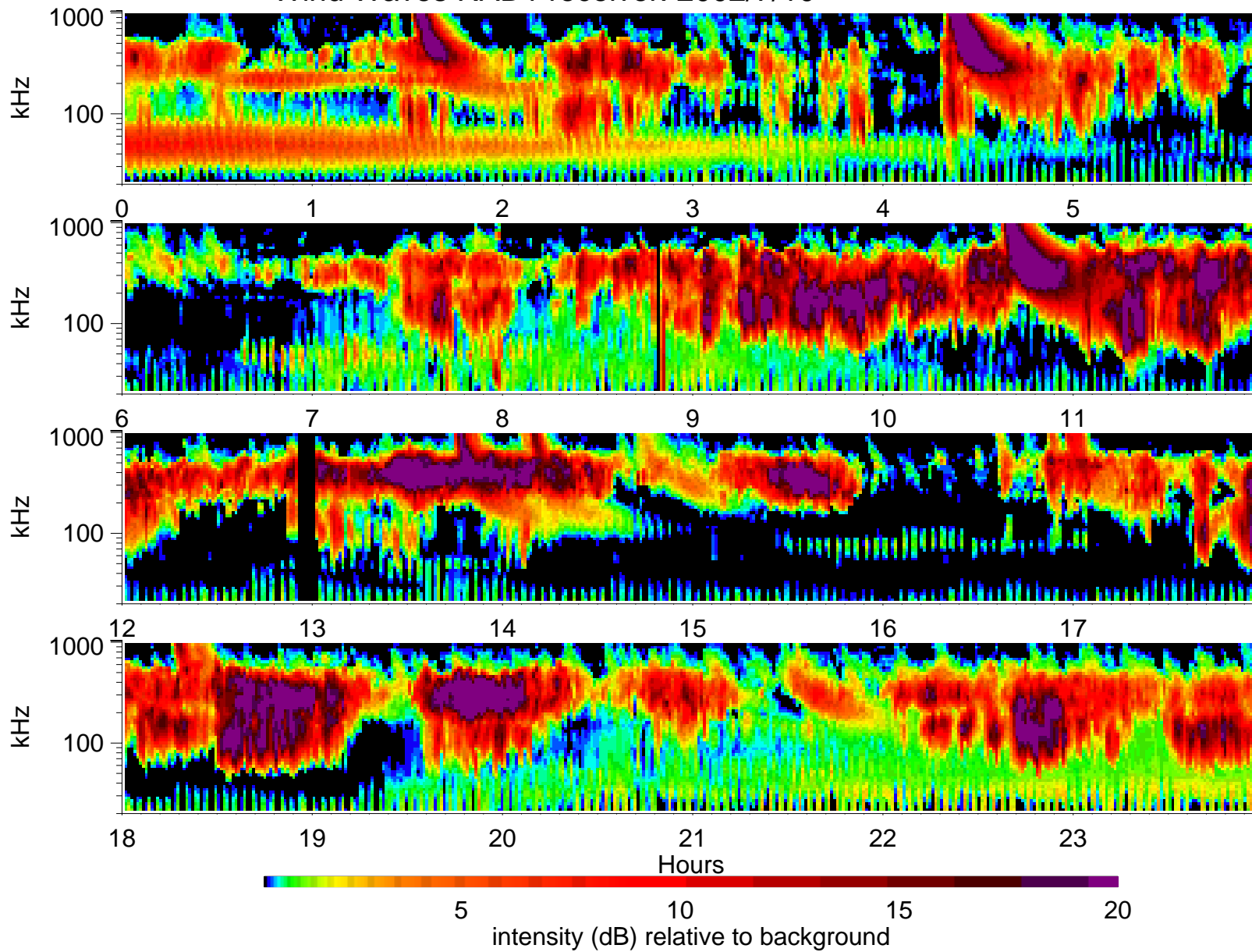
Wind Waves RAD1 receiver: 2002/7/10
