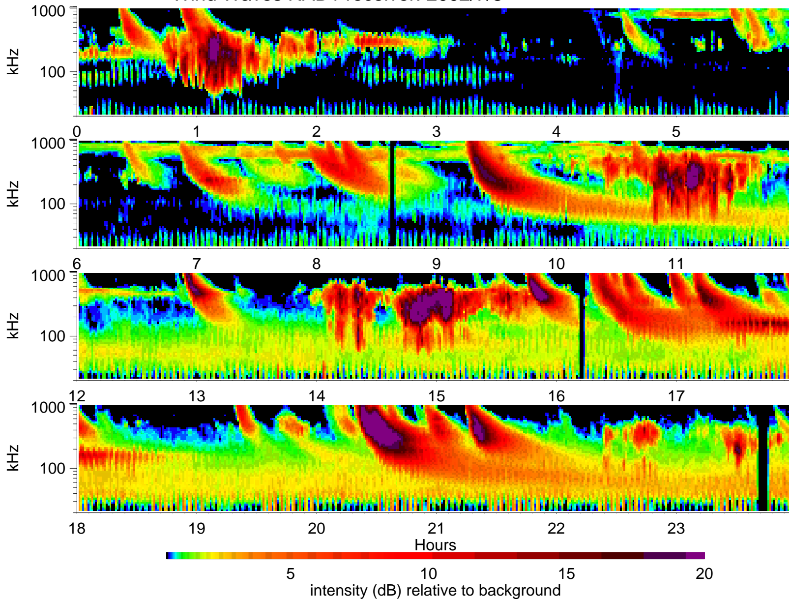
Wind Waves RAD1 receiver: 2002/7/8
