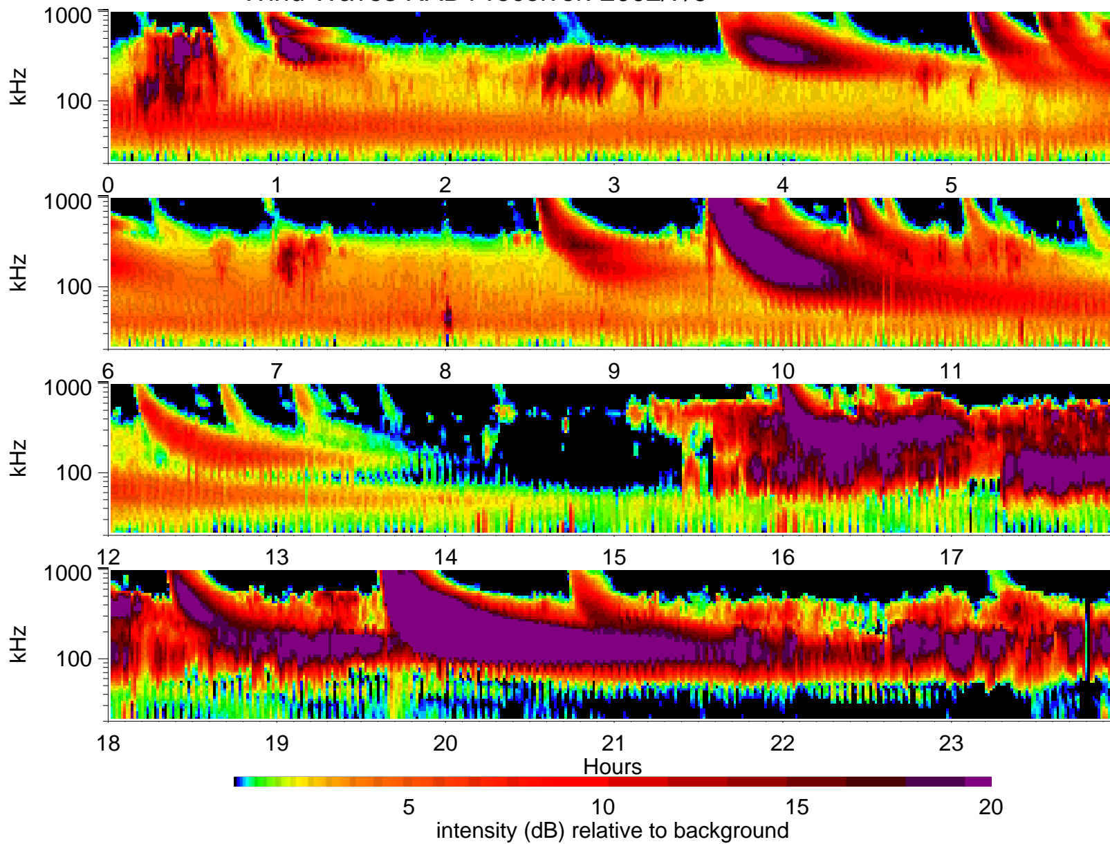
Wind Waves RAD1 receiver: 2002/7/6
