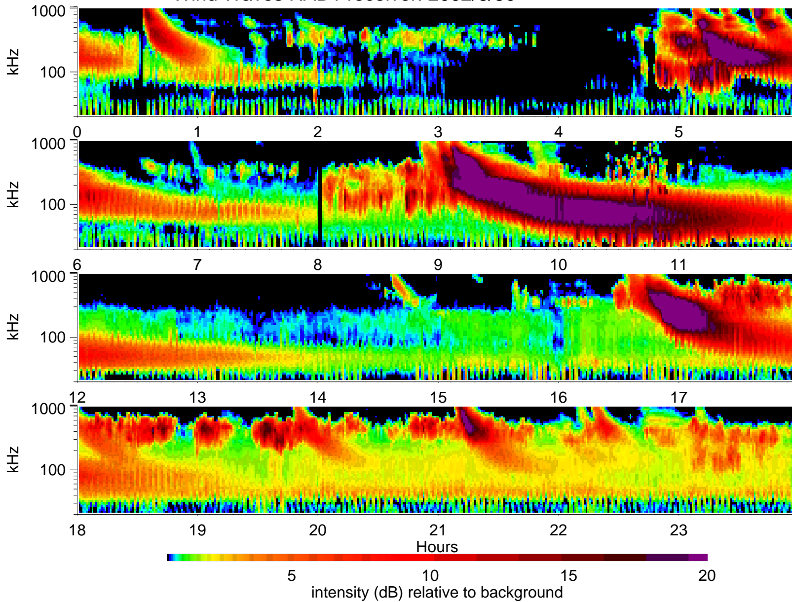
Wind Waves RAD1 receiver: 2002/6/30
