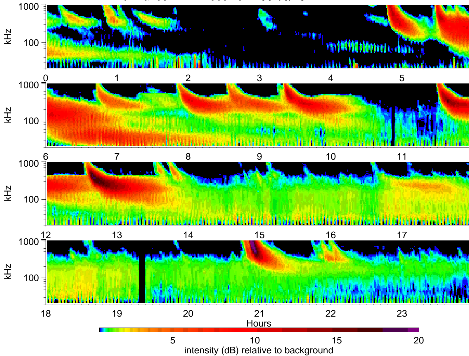
Wind Waves RAD1 receiver: 2002/6/28
