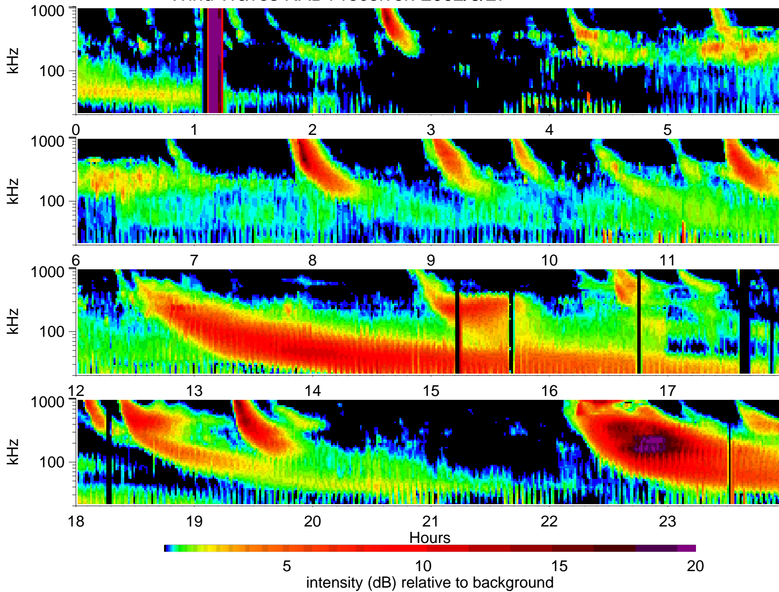
Wind Waves RAD1 receiver: 2002/6/27
