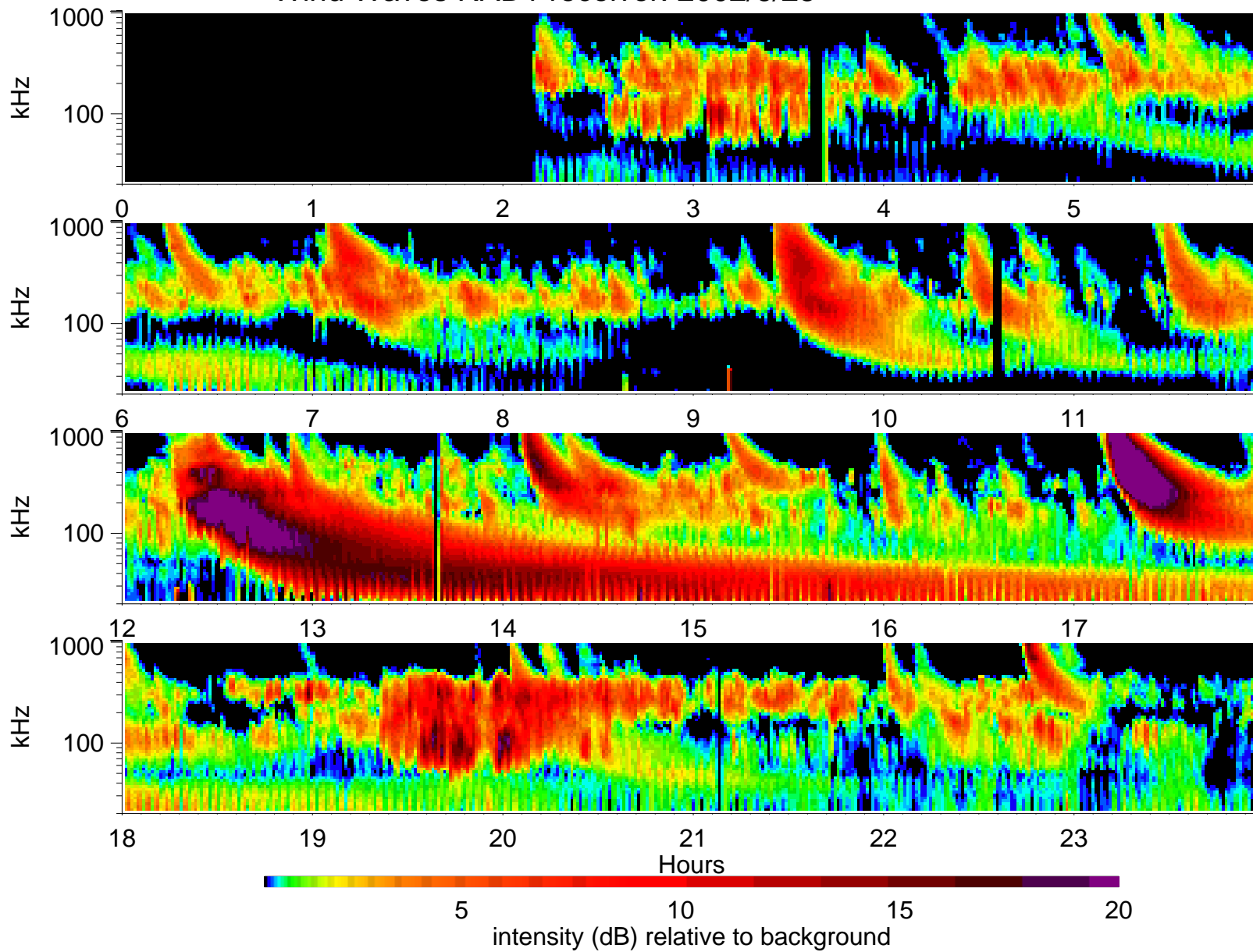
Wind Waves RAD1 receiver: 2002/6/25
