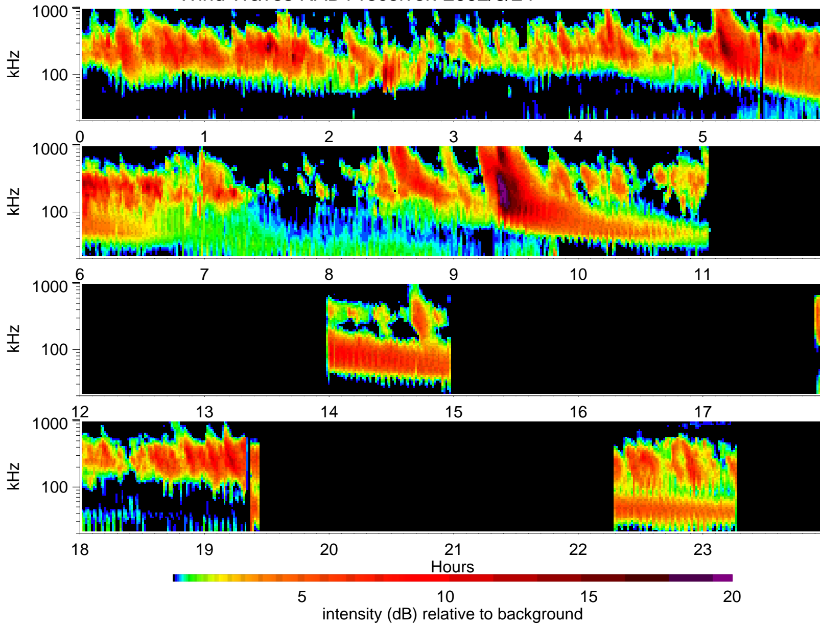
Wind Waves RAD1 receiver: 2002/6/24
