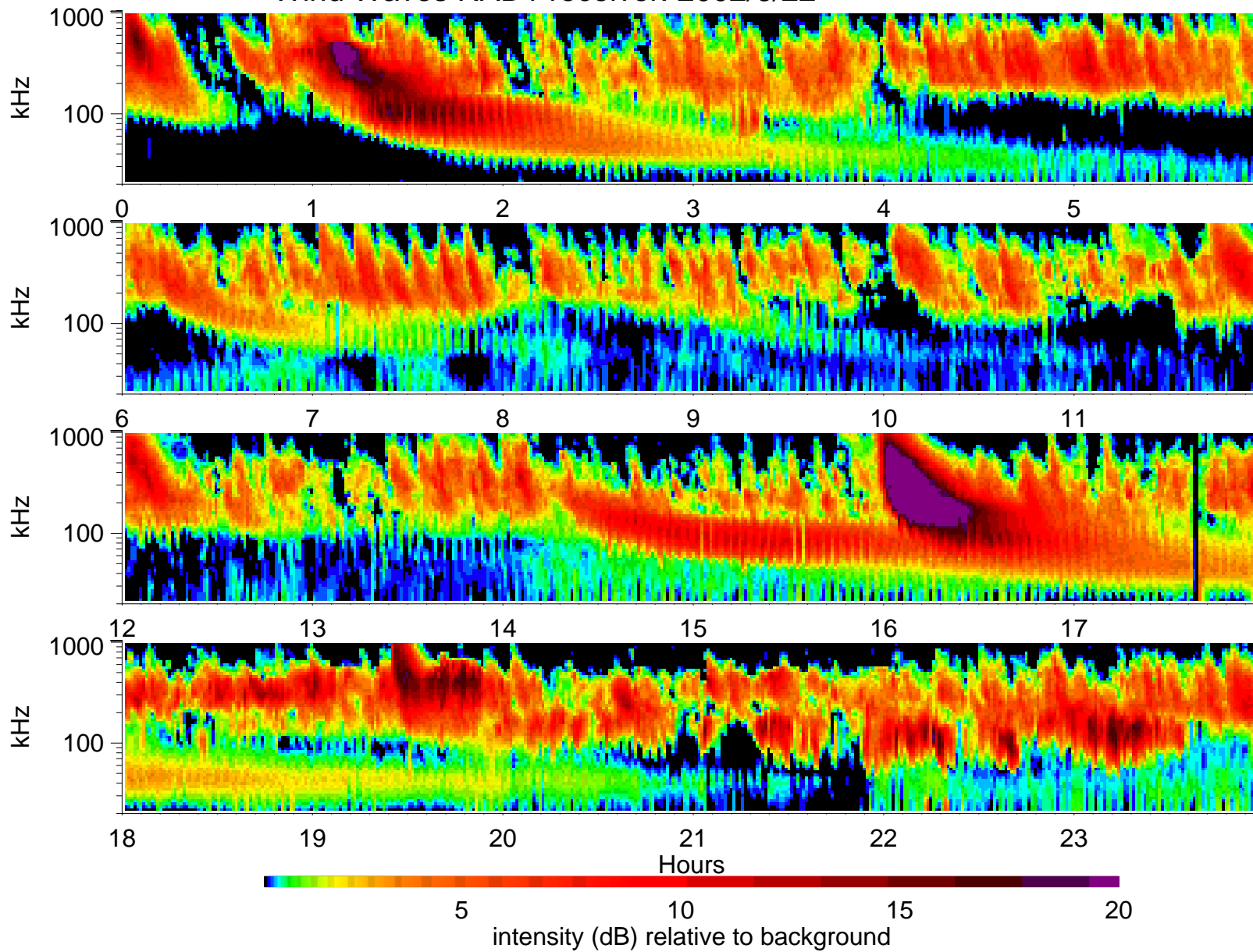
Wind Waves RAD1 receiver: 2002/6/22
