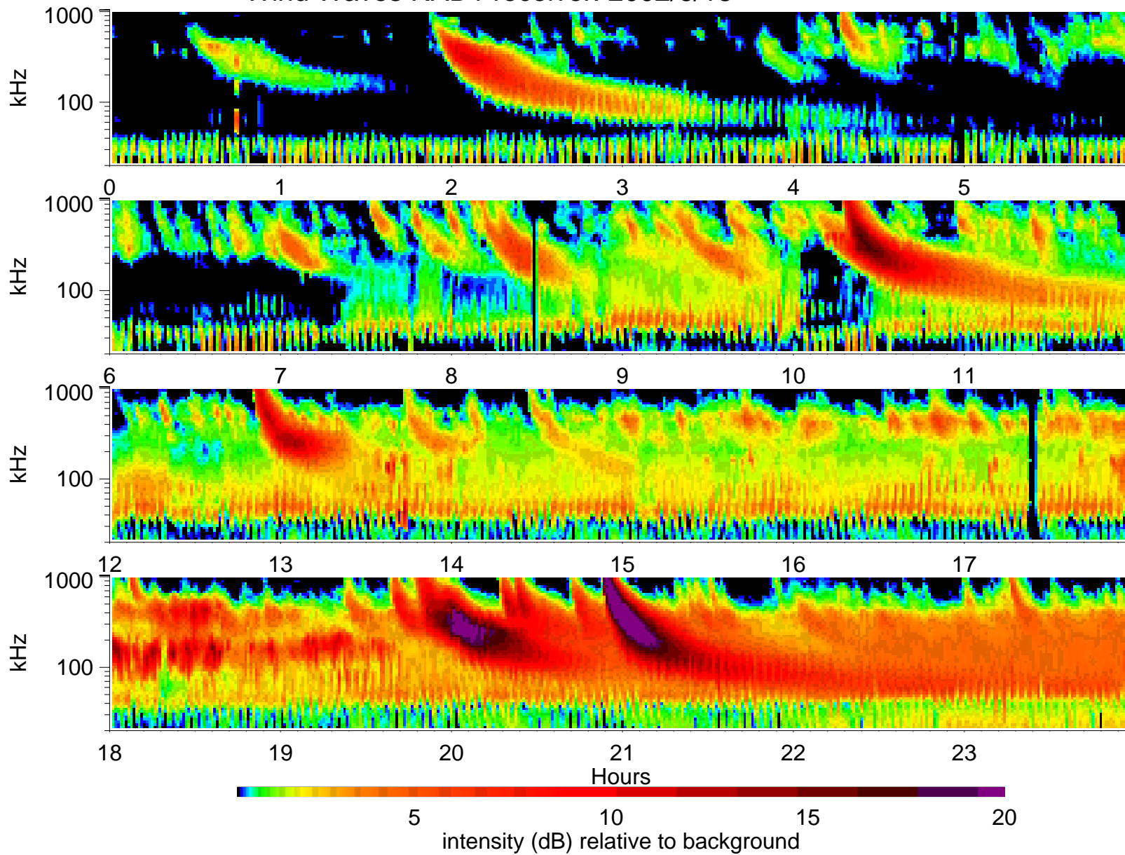
Wind Waves RAD1 receiver: 2002/6/18
