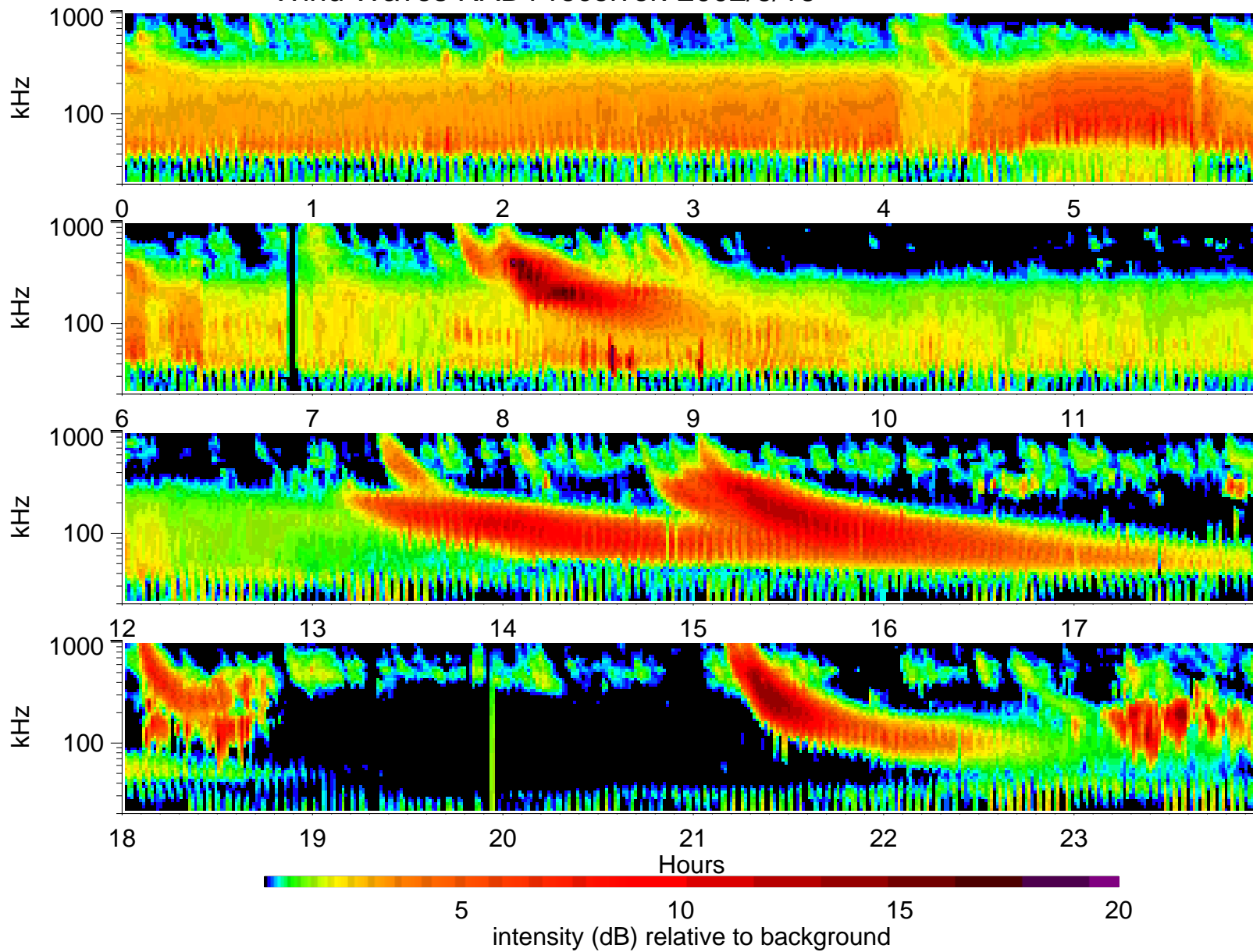
Wind Waves RAD1 receiver: 2002/6/16
