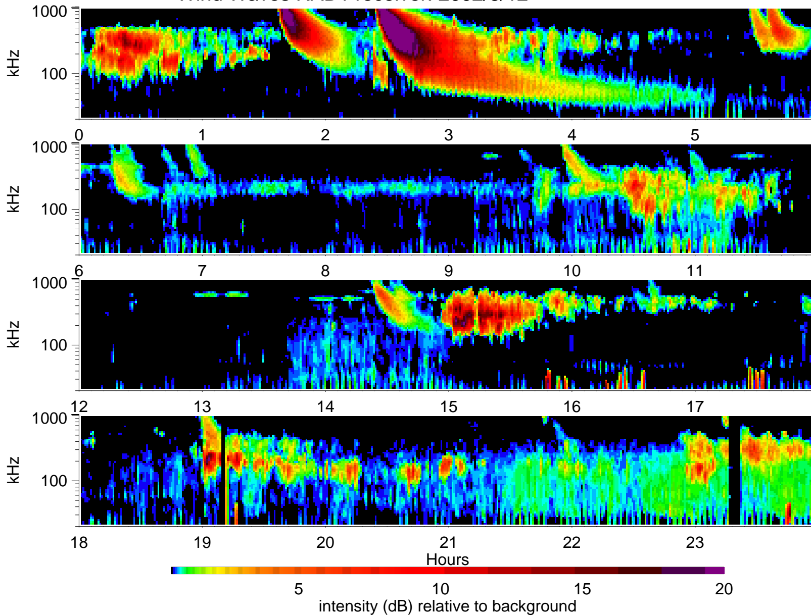
Wind Waves RAD1 receiver: 2002/6/12
