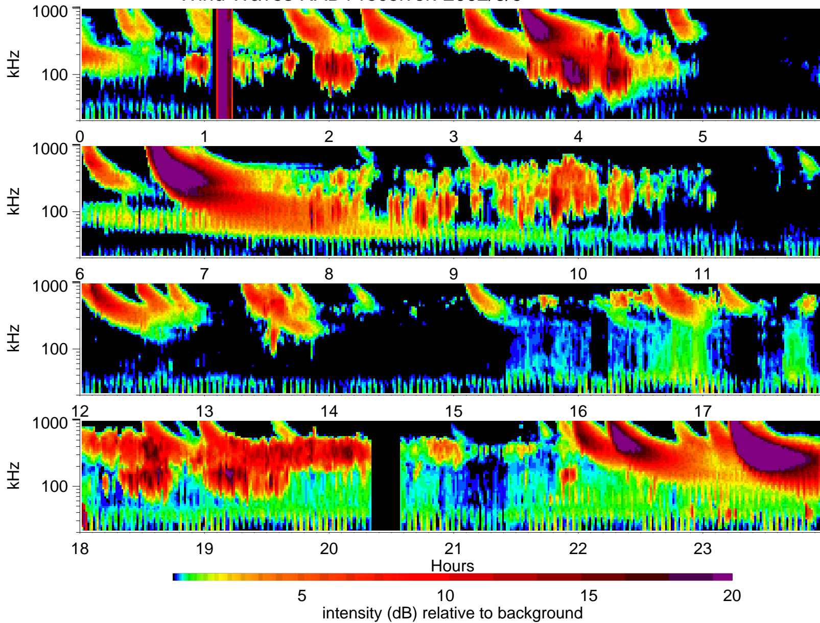
Wind Waves RAD1 receiver: 2002/6/9
