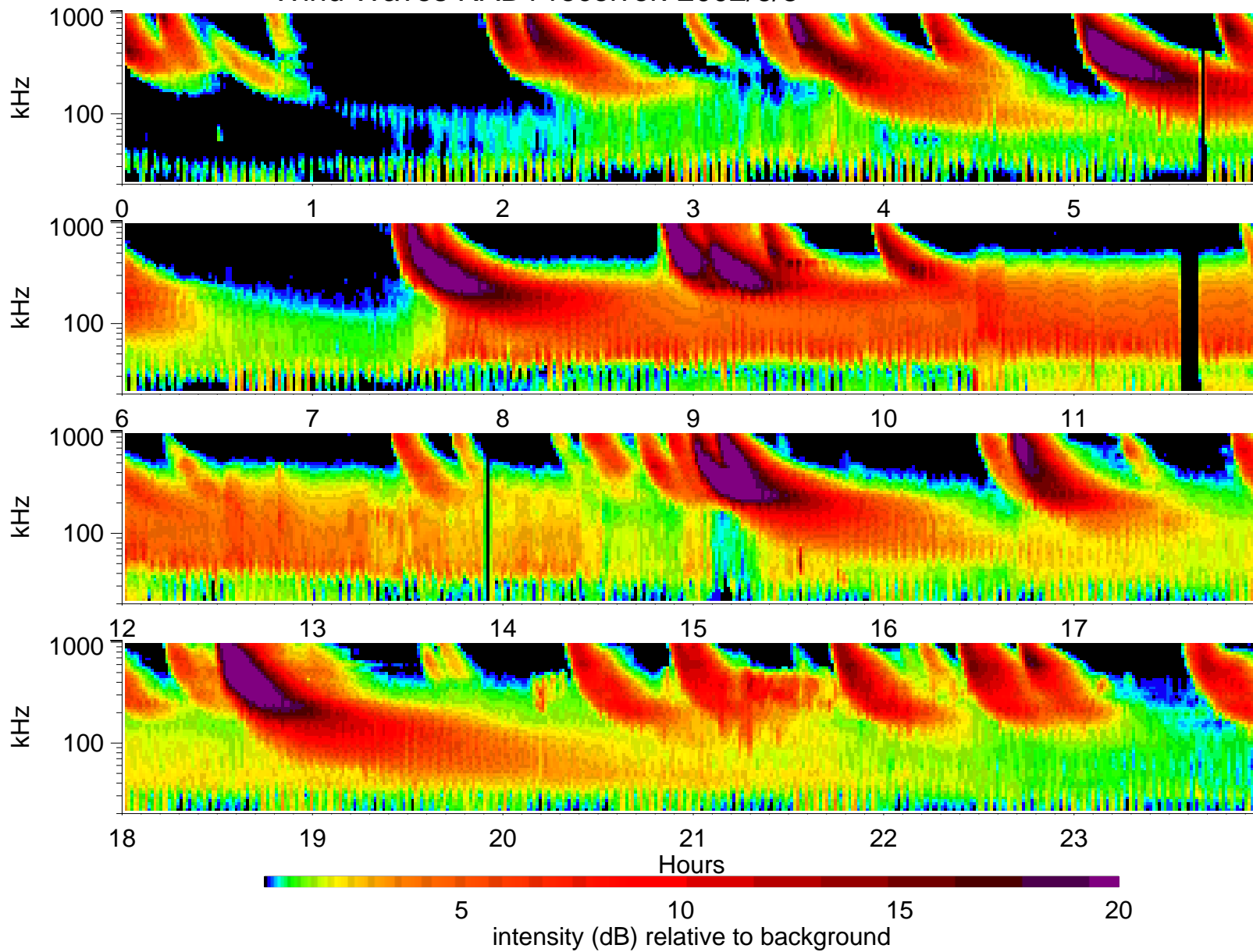
Wind Waves RAD1 receiver: 2002/6/8
