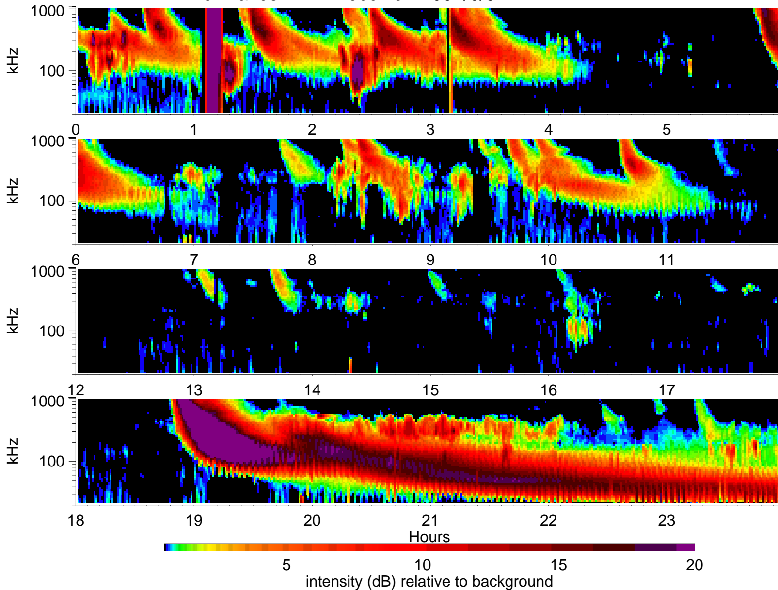
Wind Waves RAD1 receiver: 2002/6/5
