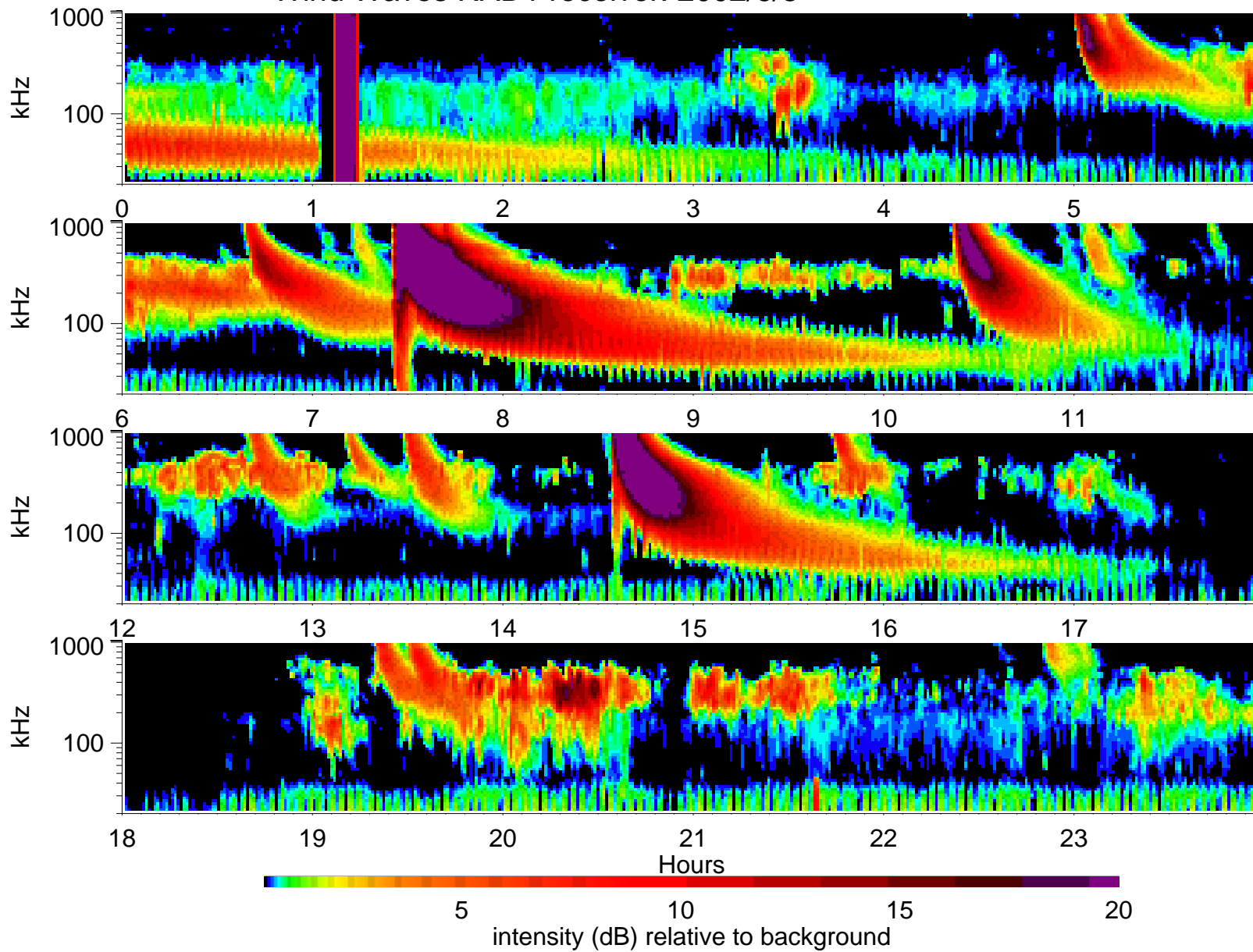
Wind Waves RAD1 receiver: 2002/6/3
