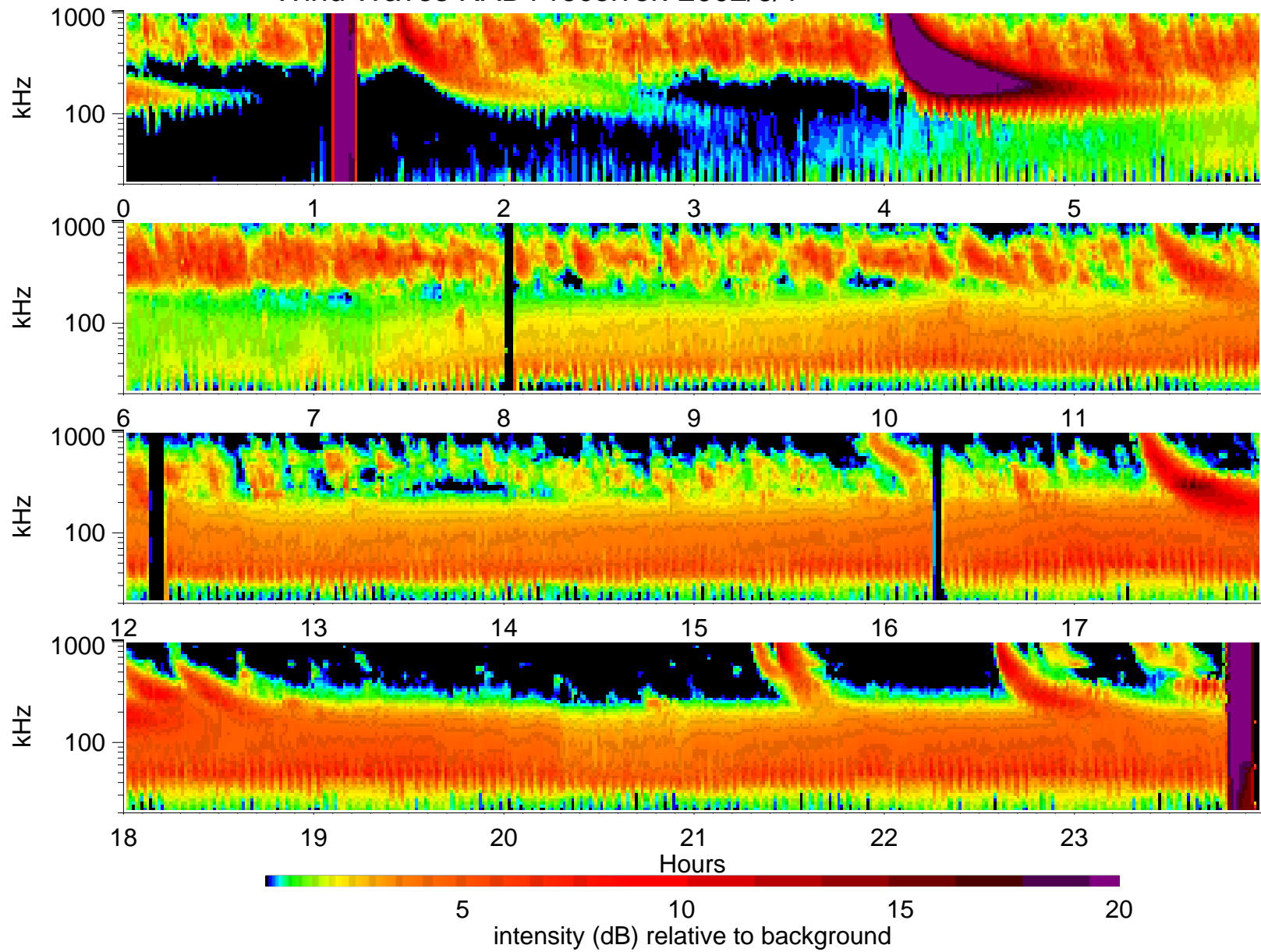
Wind Waves RAD1 receiver: 2002/6/1
