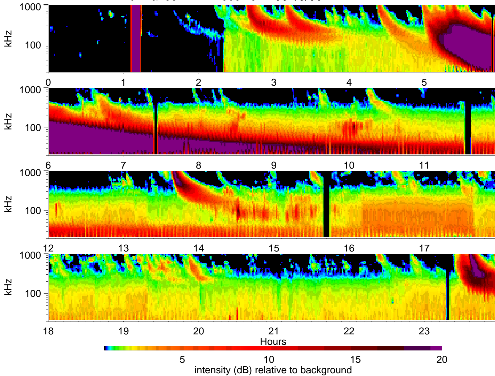
Wind Waves RAD1 receiver: 2002/5/30
