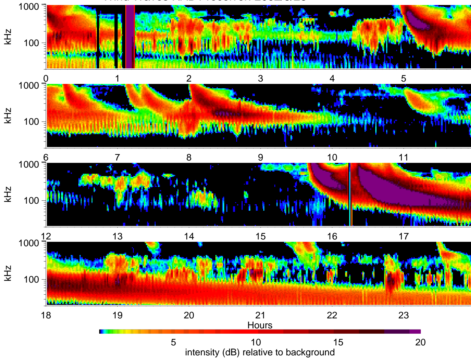
Wind Waves RAD1 receiver: 2002/5/28
