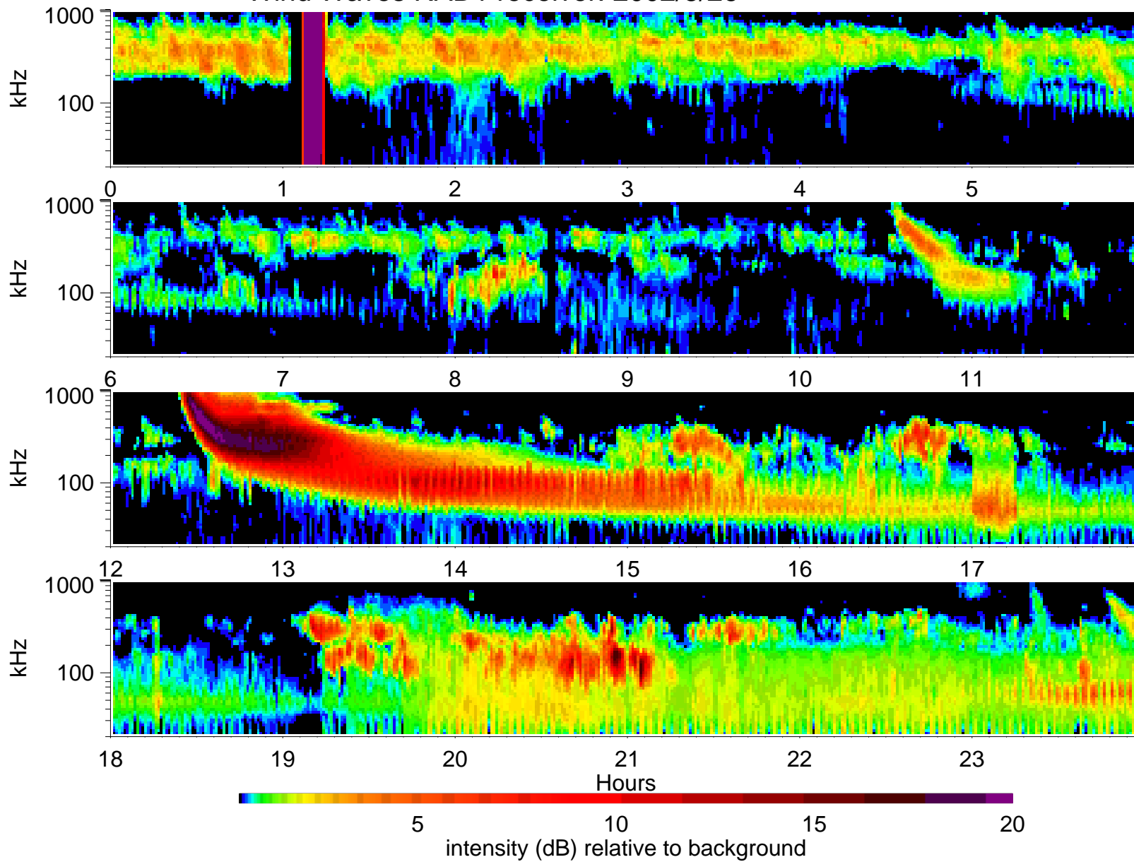
Wind Waves RAD1 receiver: 2002/5/26
