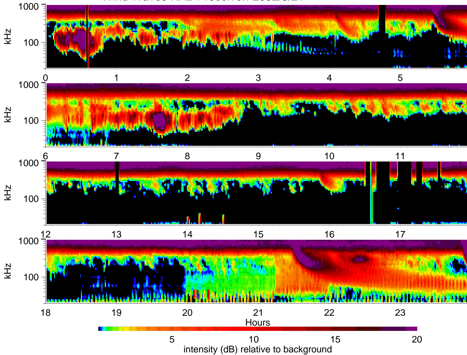
Wind Waves RAD1 receiver: 2002/5/21
