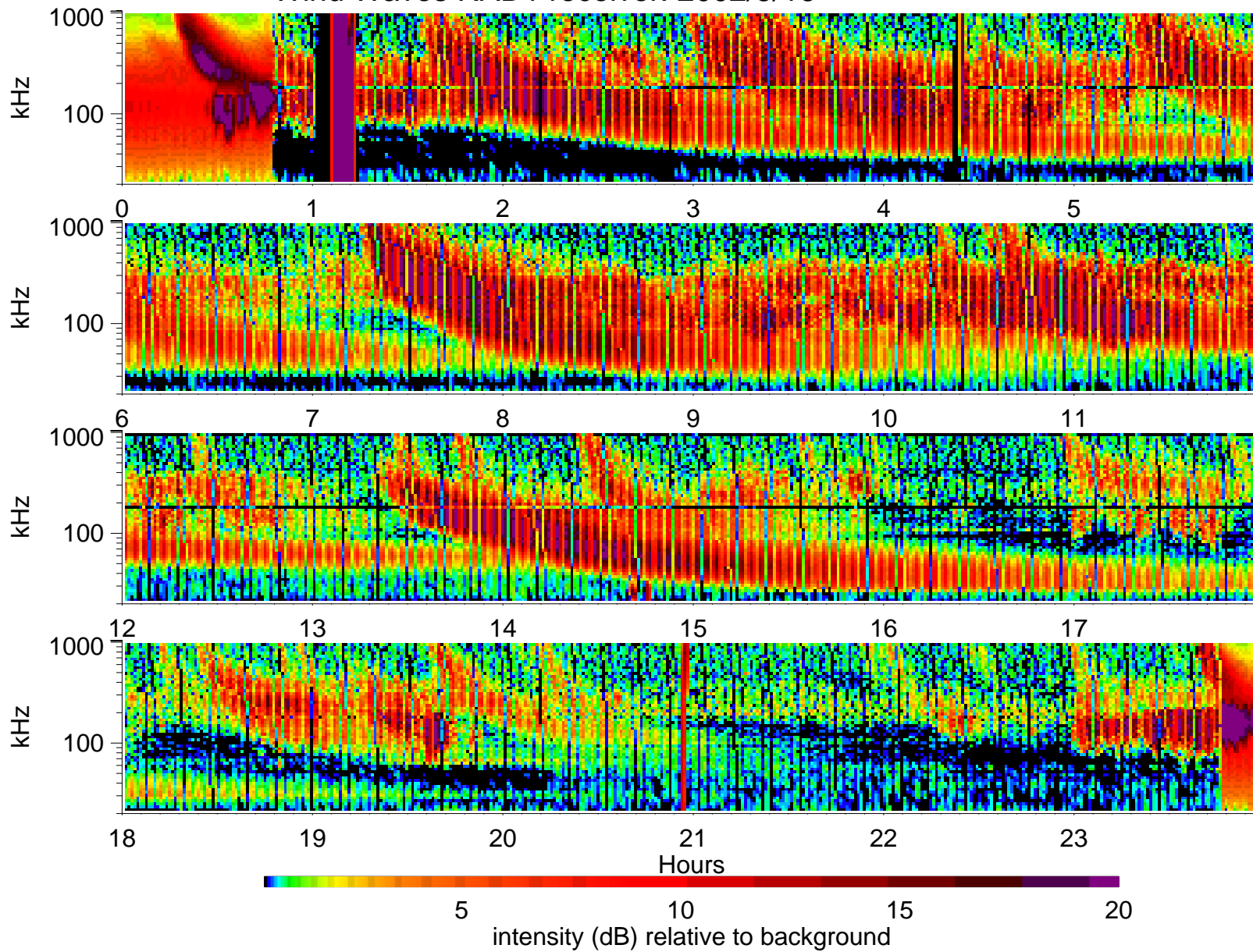
Wind Waves RAD1 receiver: 2002/5/16
