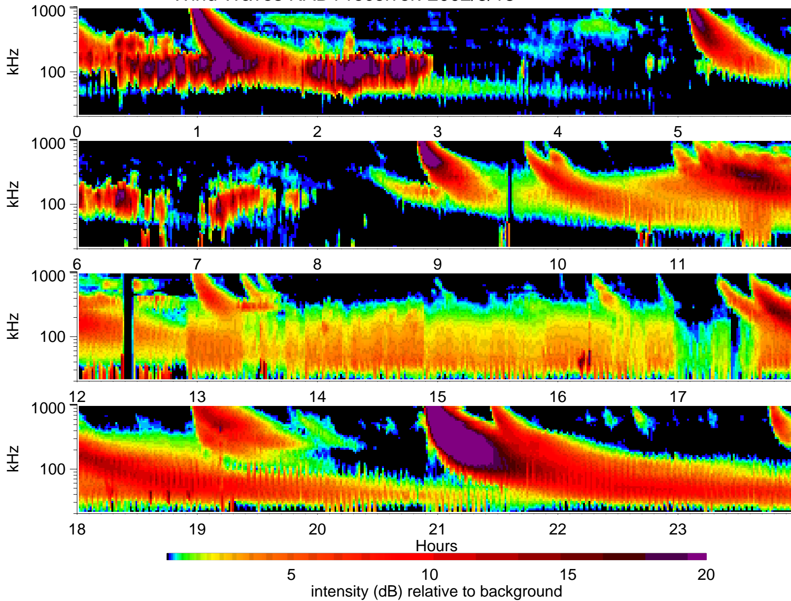
Wind Waves RAD1 receiver: 2002/5/13
