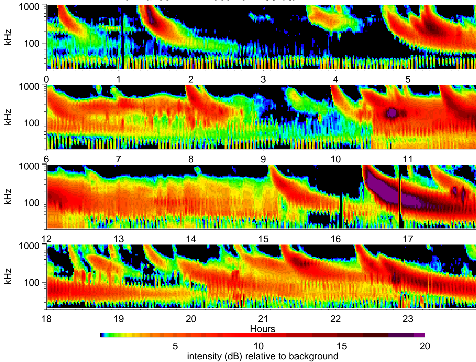
Wind Waves RAD1 receiver: 2002/5/11
