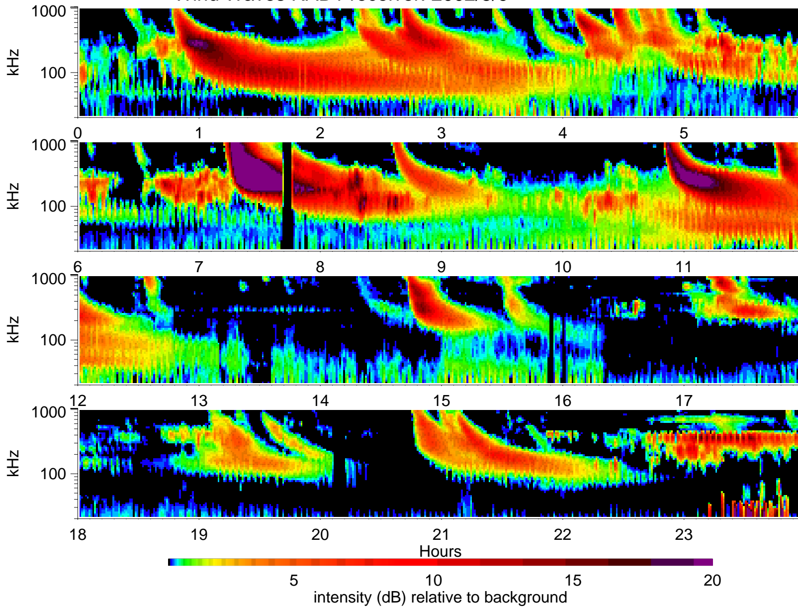
Wind Waves RAD1 receiver: 2002/5/9
