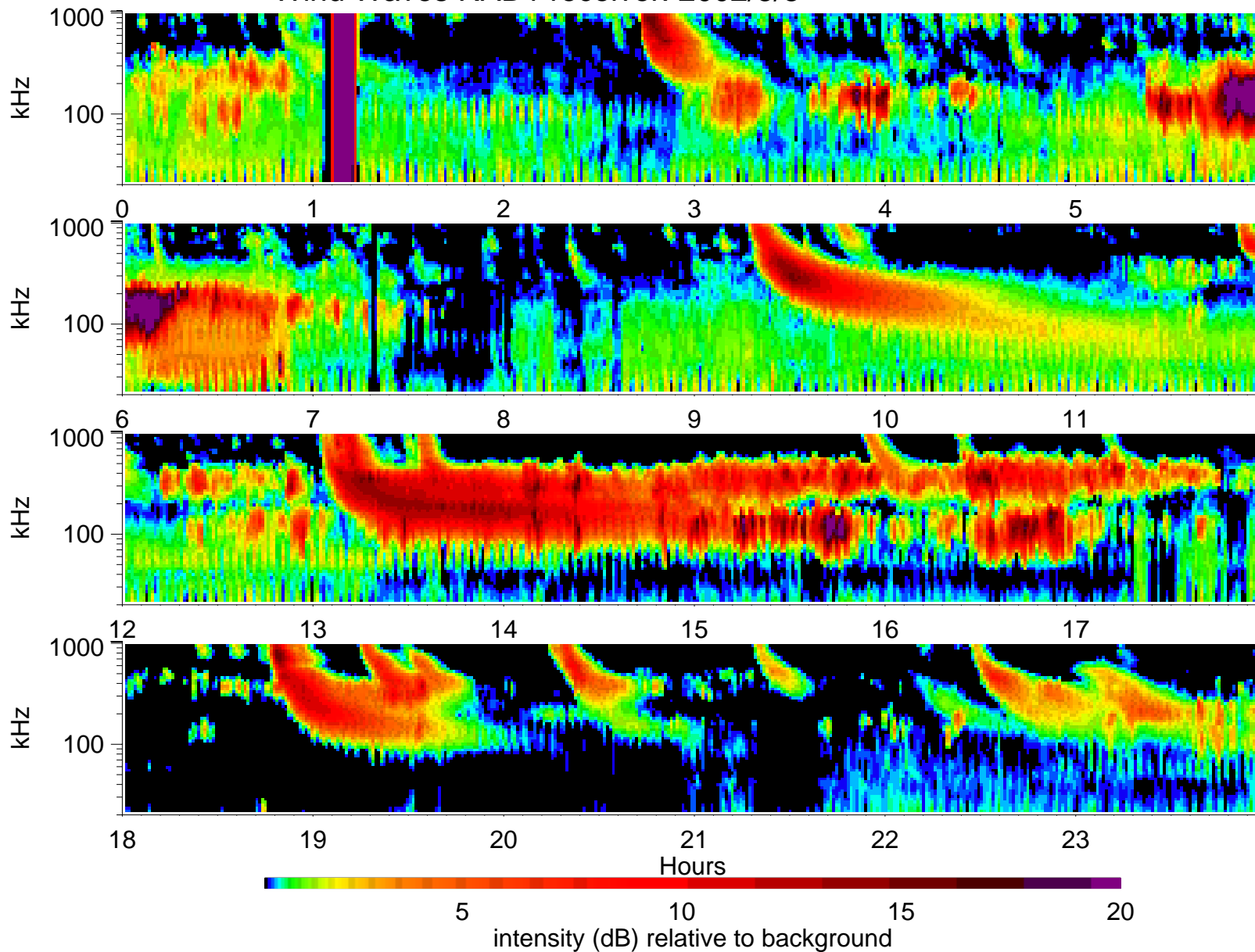
Wind Waves RAD1 receiver: 2002/5/8
