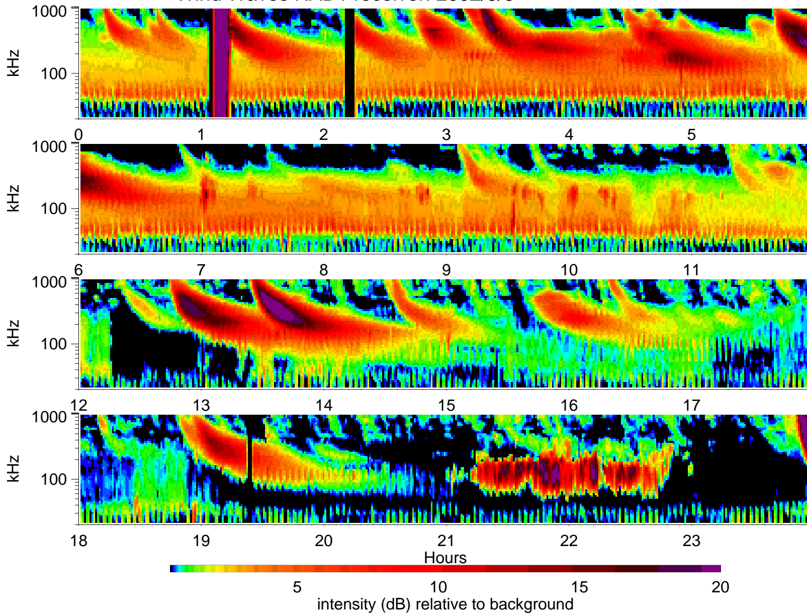
Wind Waves RAD1 receiver: 2002/5/6
