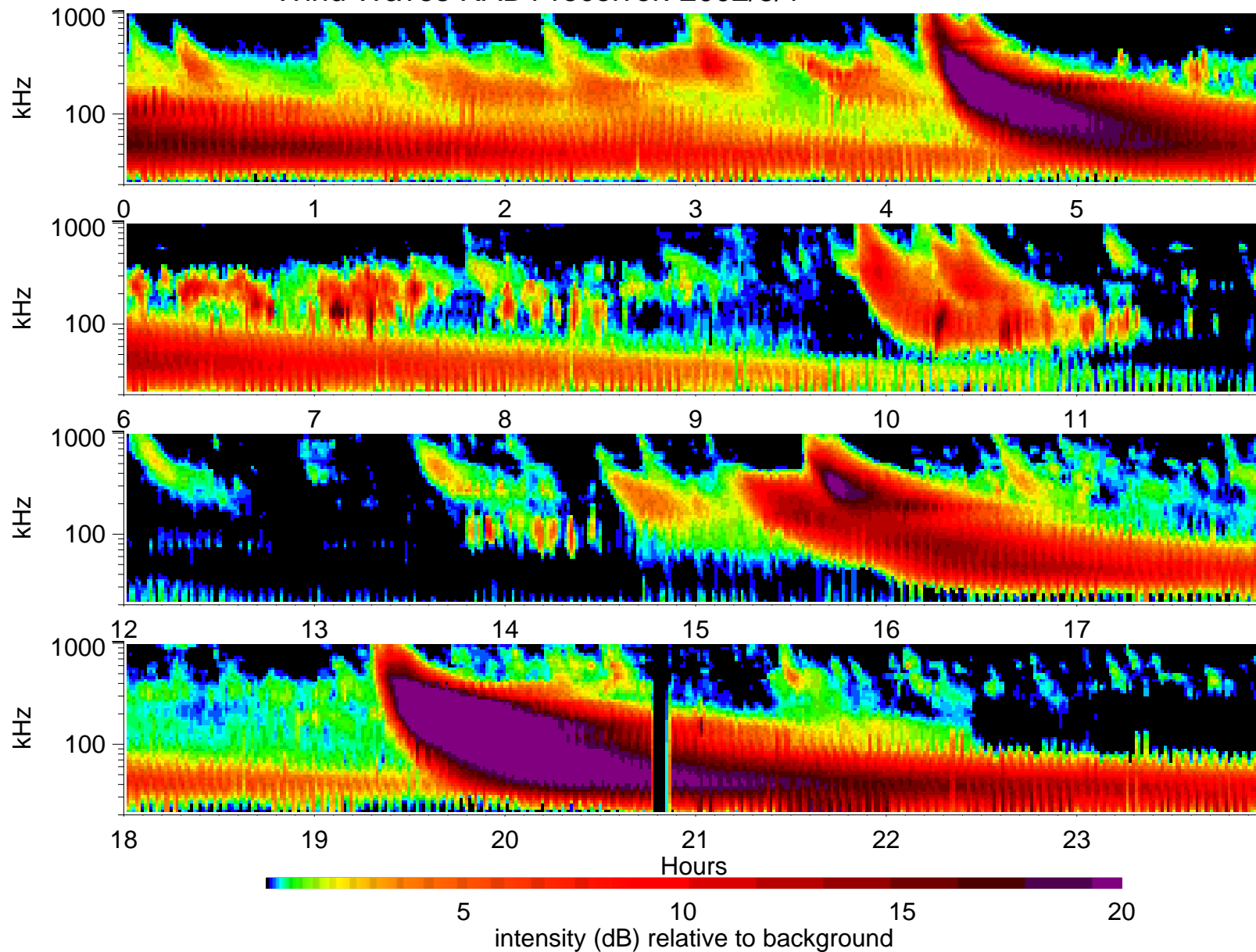
Wind Waves RAD1 receiver: 2002/5/1
