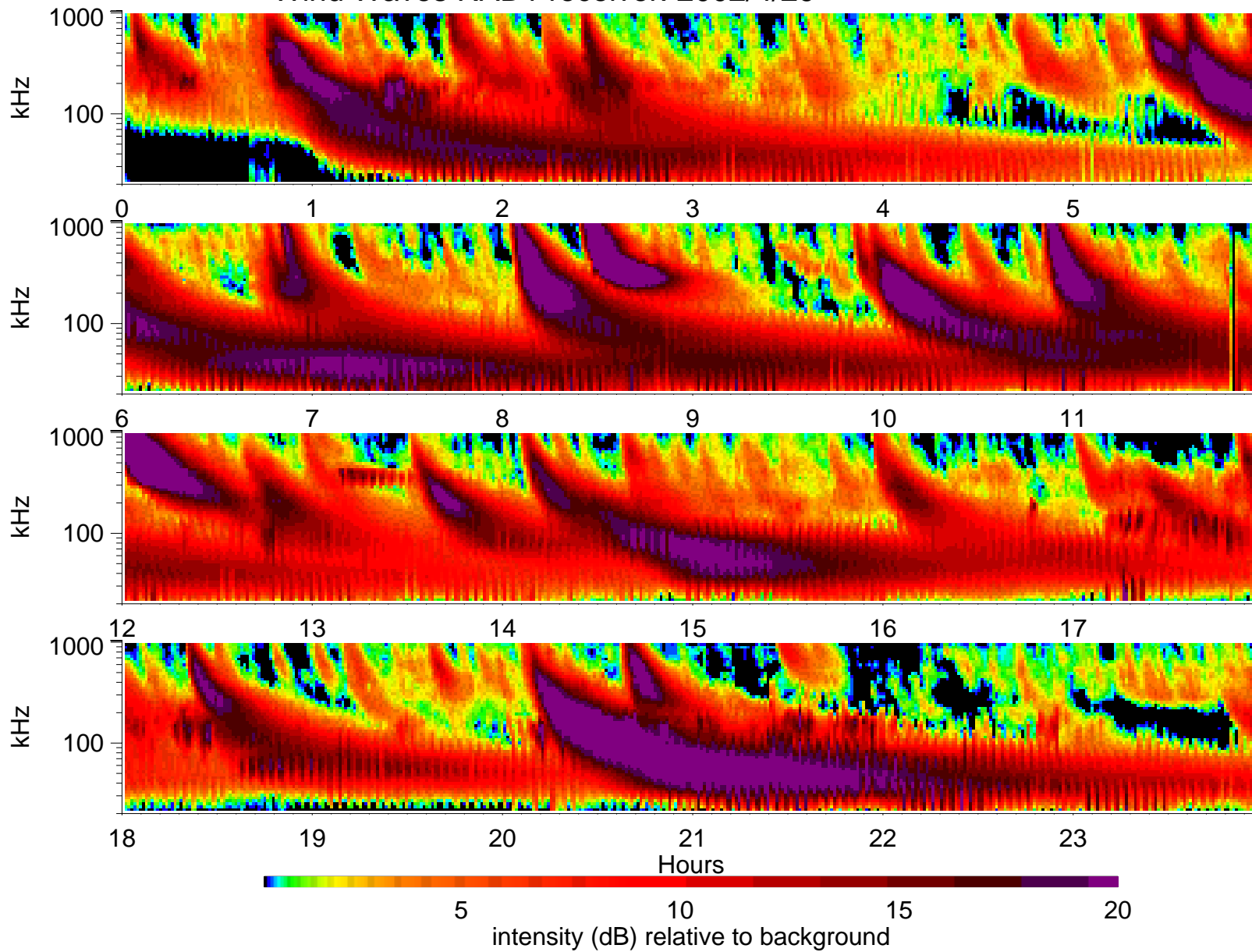
Wind Waves RAD1 receiver: 2002/4/29
